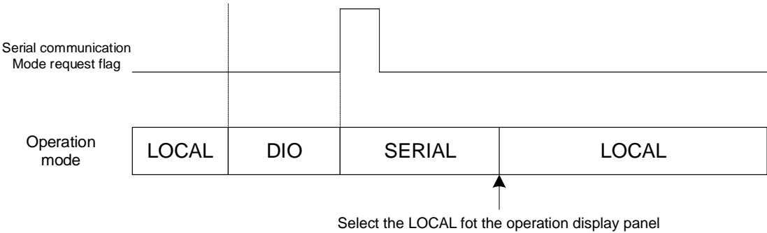
Fig.1-1 Operation mode
