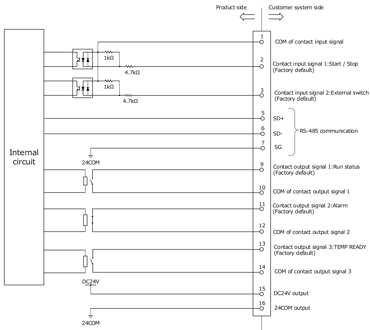
Fig.2-1 Circuit diagram
