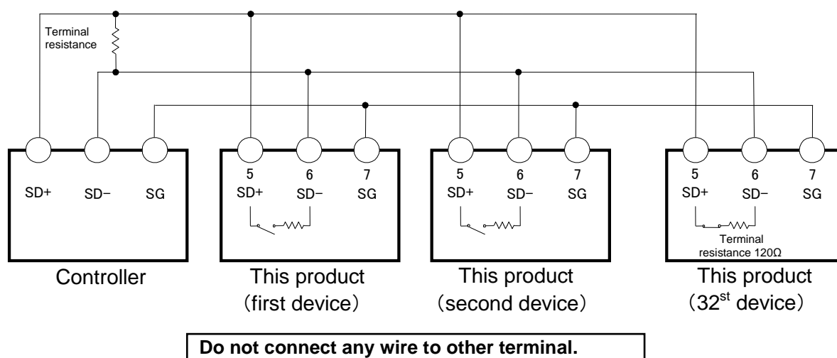
Fig.3-1 RS-485 connection
