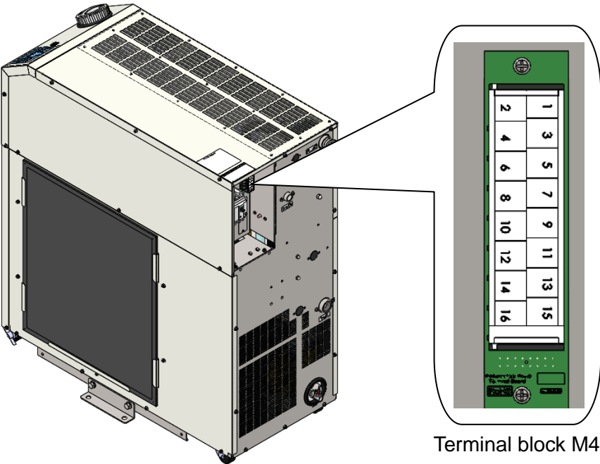
Fig.1-3 Communication port
