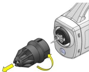
Nozzle removal
