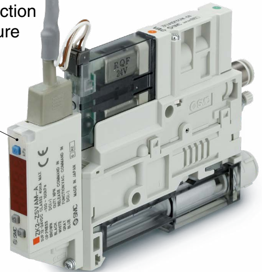
Digital pressure switch for vacuum with energy-saving function
